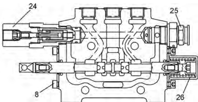
"E-E" SECTION
