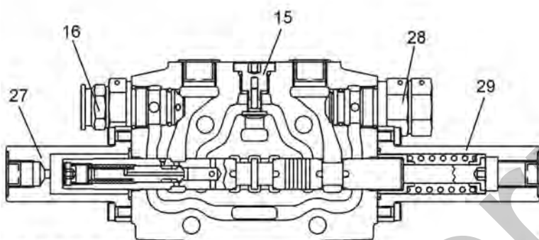
"F-F" SECTION
