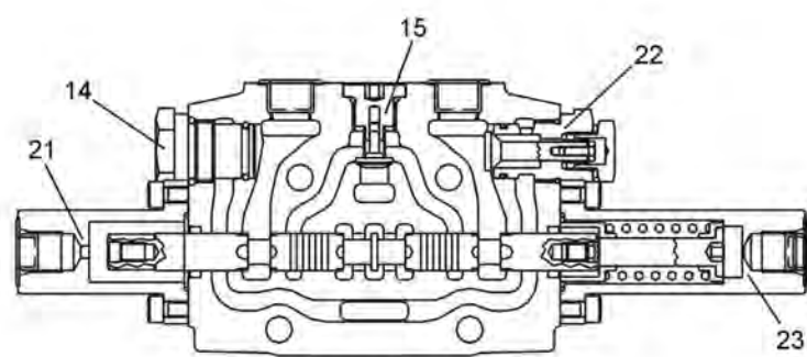
"D-D" SECTION
