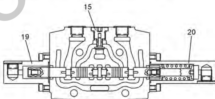
"C-C" SECTION
