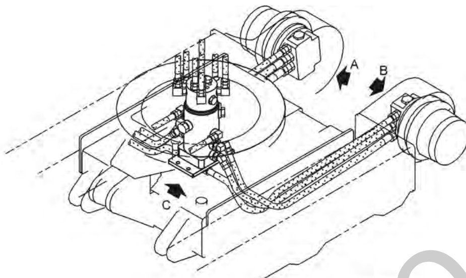
"A" DETAIL
