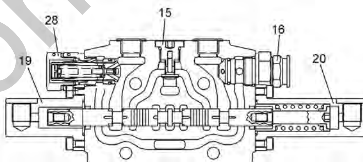
"I-I" SECTION
