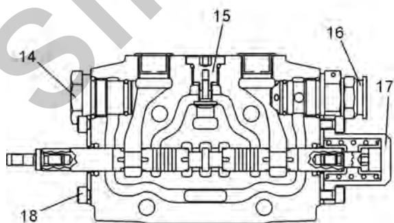
"B-B" SECTION
