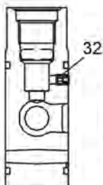
"M-M" SECTION
